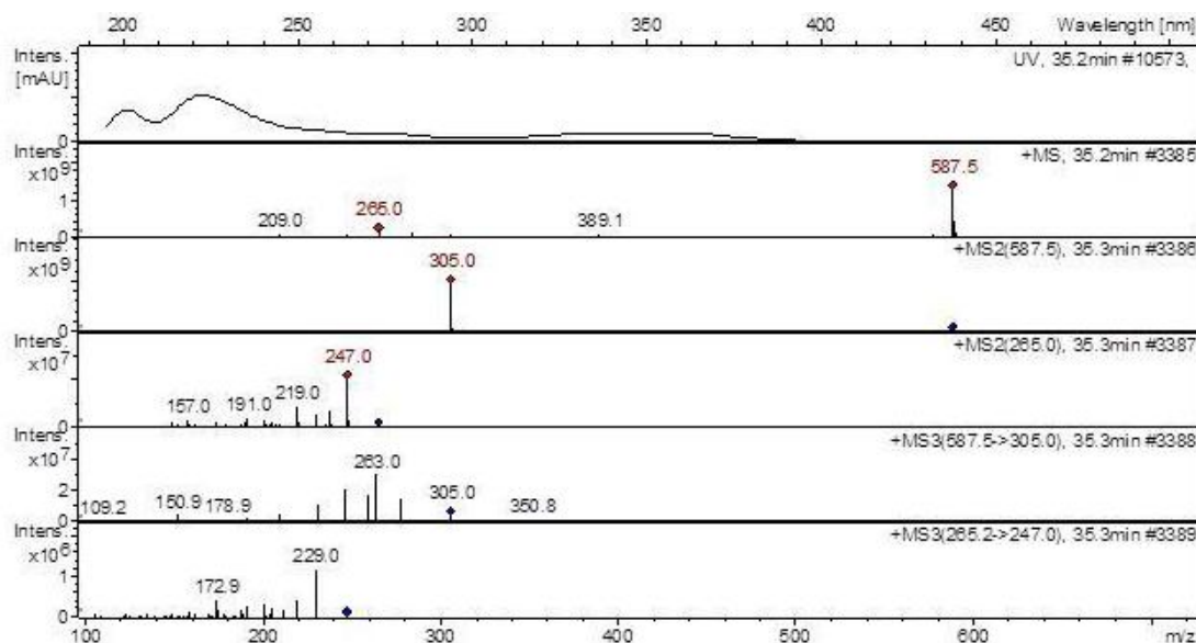
Fig. 2: The HPLC/DAD/MS3 mass spectra and fragmentation pattern of artemisinin peak present in the methanolic extract of A. annua as well as that of artemisinin standard.
