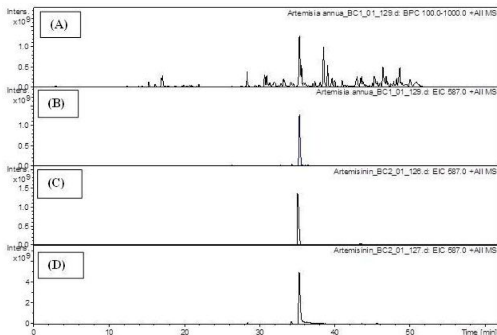
Fig. 4 (A): Typical HPLC-positive mode ESI-MSn base peak chromatogram (BPC) profile of the methanolic extract of Artemisia annua showing artemisinin peak as the major active ingredient.
