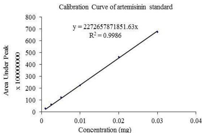
Fig. 3: Calibration Curve of Artemisinin obtained by six levels of concentrations of standard, with three injections per level.
