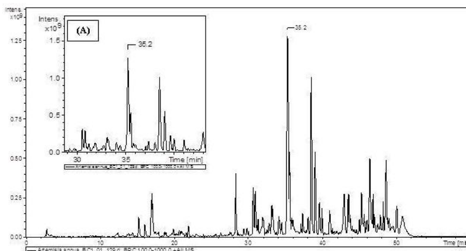
Fig. 1(A): Typical HPLC-positive mode ESI-MSn base peak chromatogram (BPC) profile of the methanolic extract of Artemisia annua showing artemisinin peak eluted at 35.2 min as the major active ingredient.
